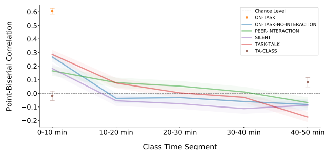
Figure 6: Point-biserial correlation coefficients with 95% confidence intervals by class segment for the onset features model.
